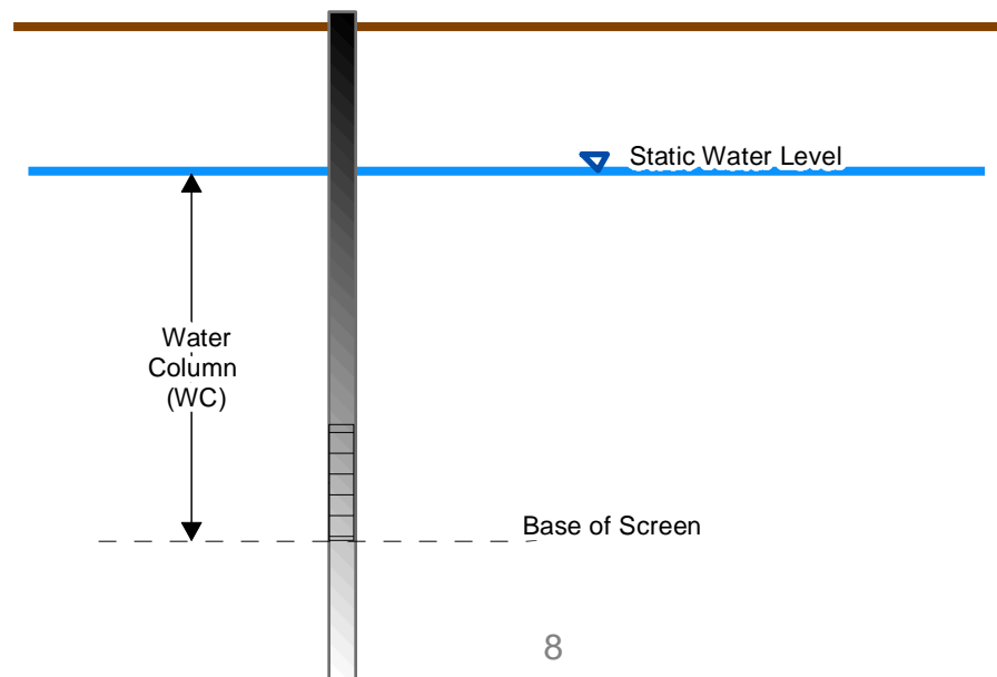
Case 3: Case Where Water Column Limited by Base of Screen Interval
