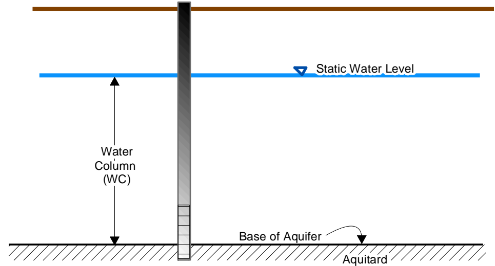
Case 2: Case Where Water Column Limited by Base of Aquifer
