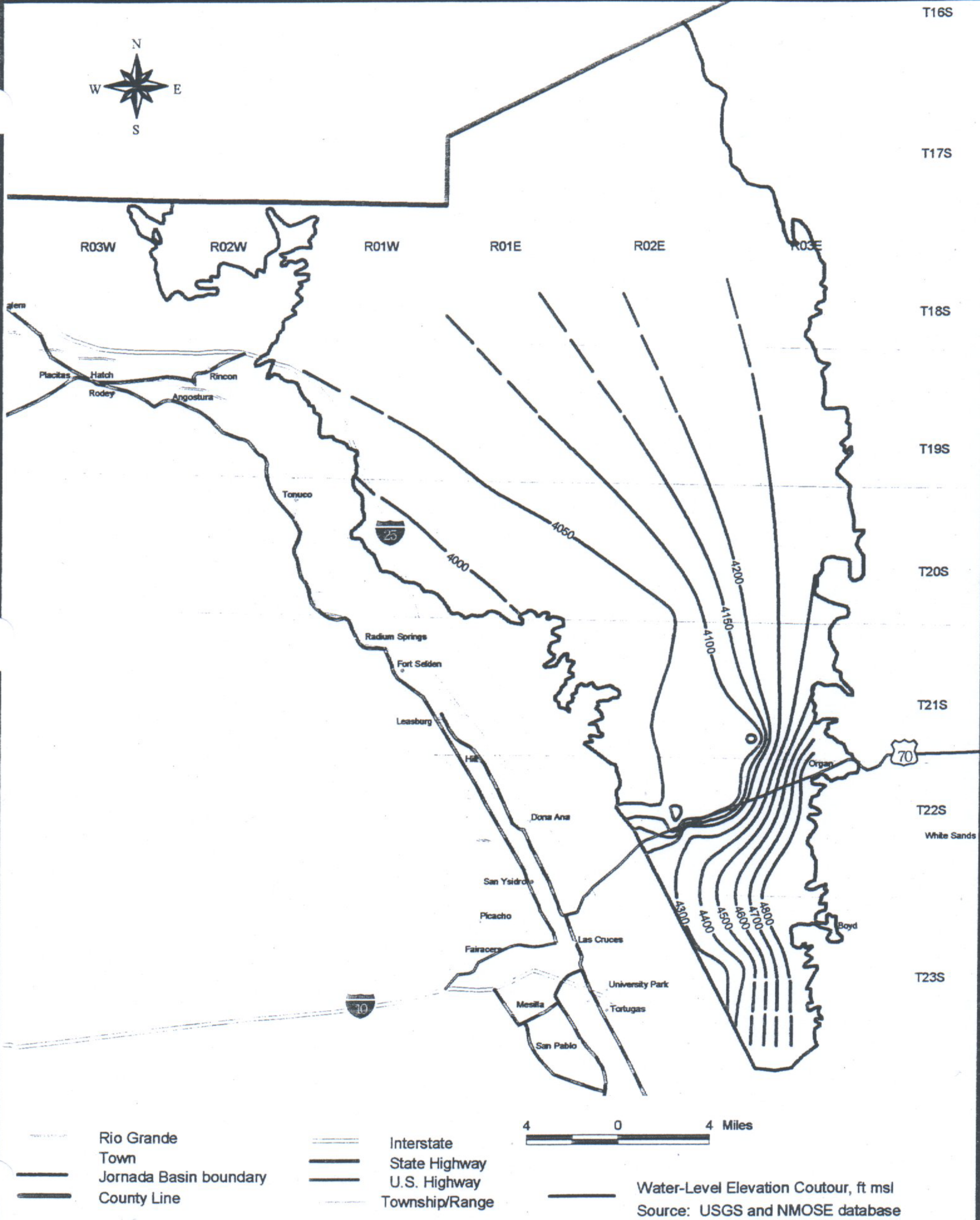
Figure 6.29 Map showing water-level elevation contours, 1978-1983, Jornada Basin, Dona Ana County, New Mexico.
