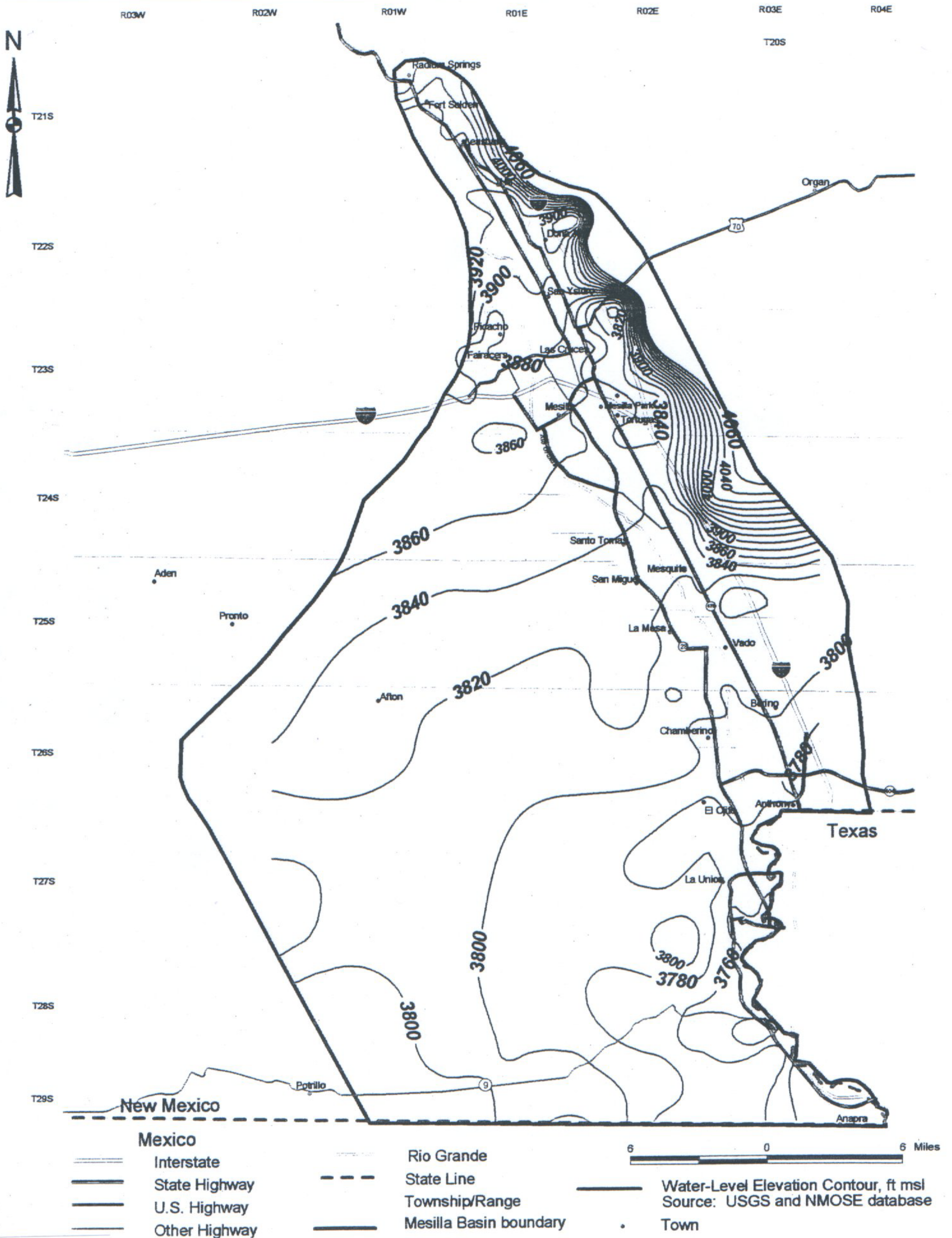
Figure 6.25 Map showing water-level elevation contours, 1995-2000, Mesilla Basin, Dona Ana County, New Mexico.
