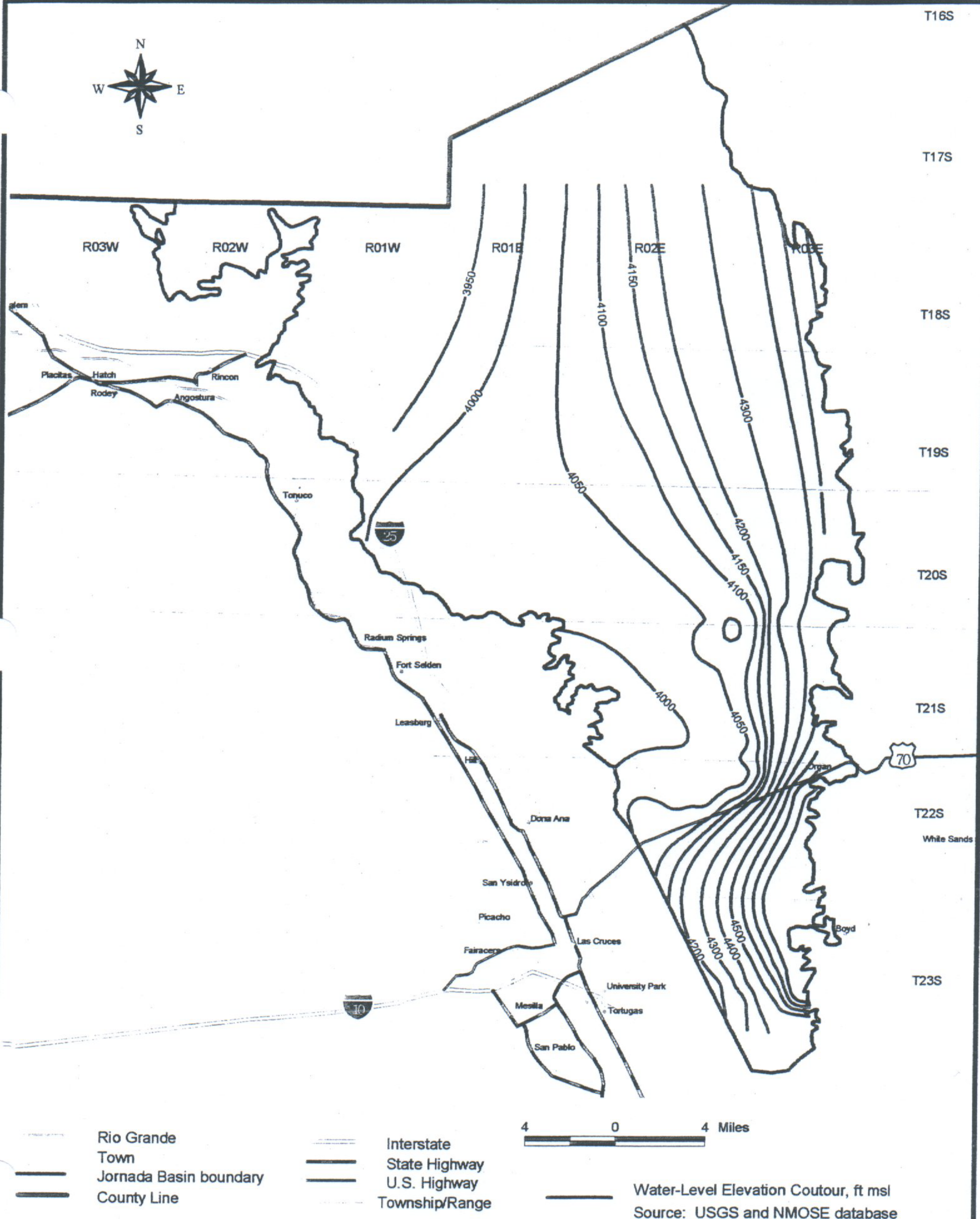
Figure 6.30 Map showing water-level elevation contours, 1995-2000, Jornada Basin, Dona Ana County, New Mexico.
