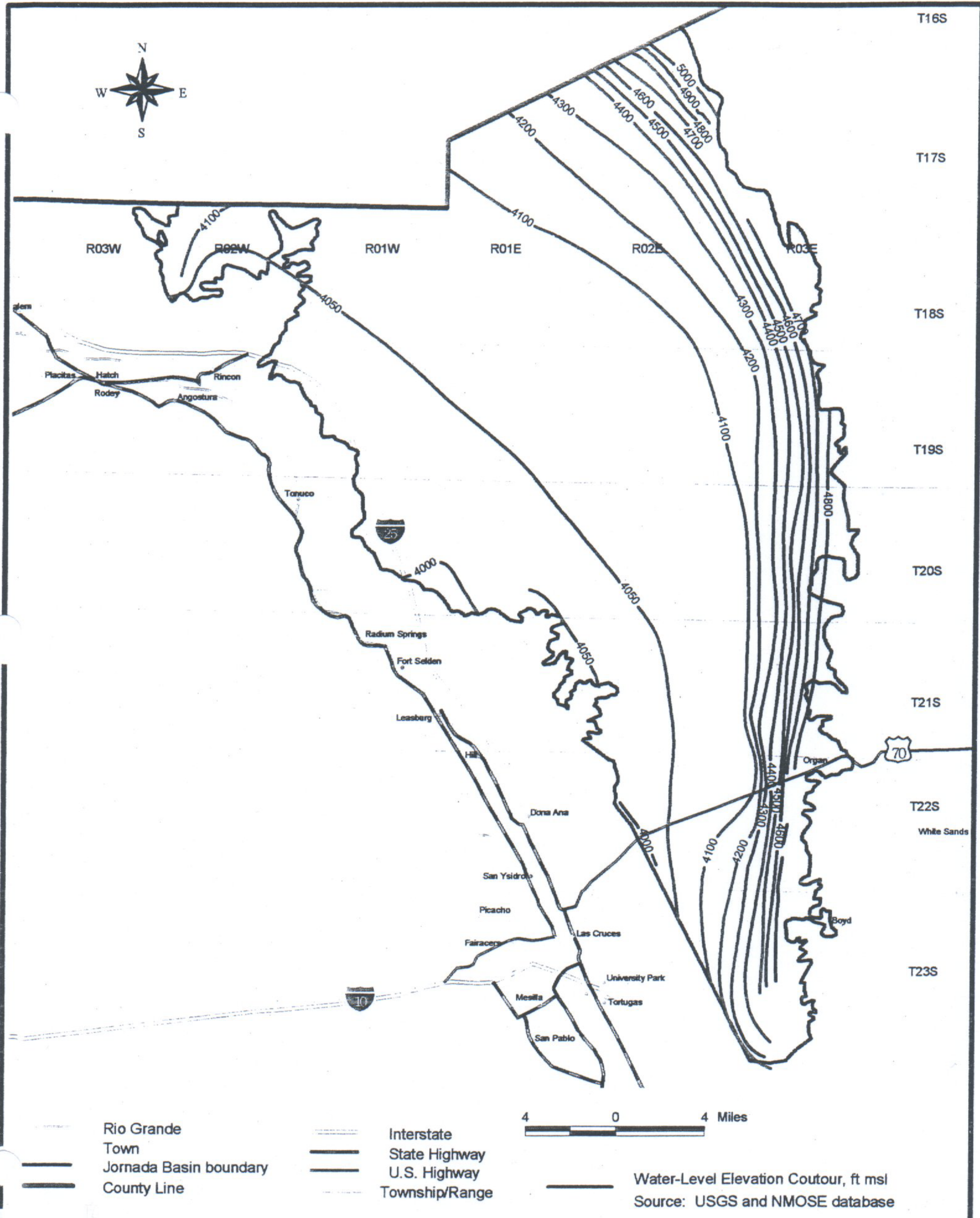
Figure 6.28 Map showing water-level elevation contours, pre-1970 development, Jornada Basin, Dona Ana County, New Mexico.
