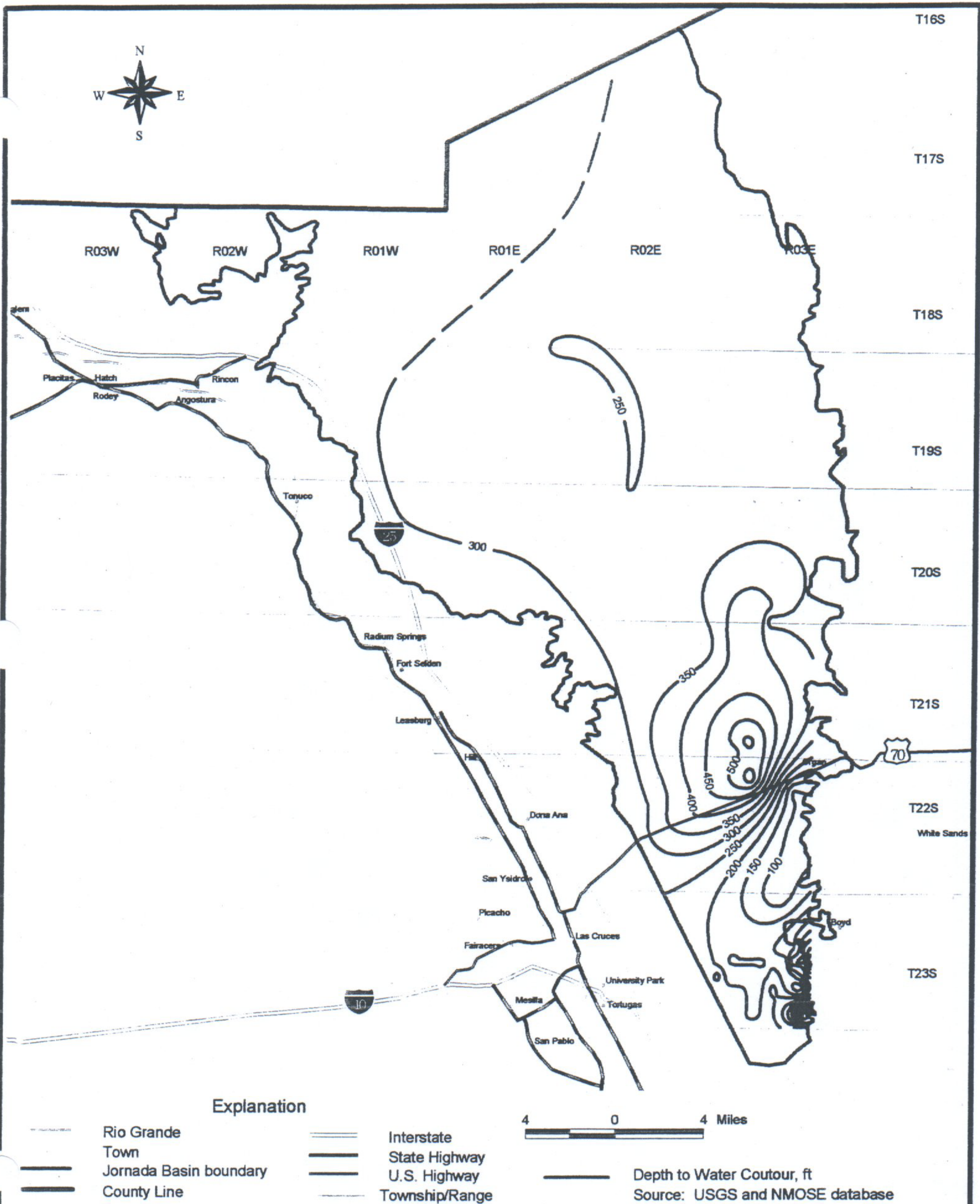
Figure 6.27 Map showing depth to water contours, 1995-2000, Jornada Basin, Dona Ana County, New Mexico.
